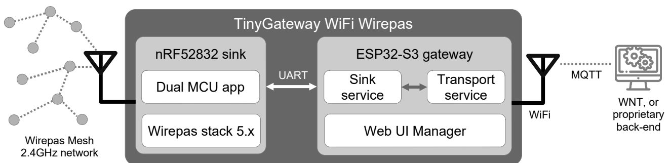
TinyGateway WiFi Wirepas: architecture and interfaces
